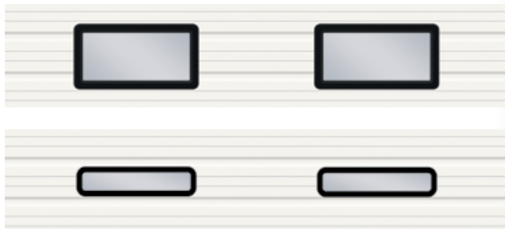
Windows: 25" x 13" or 24" x 6". Glass: ½" Clear, double-pane or ⅛" Clear, single-pane. Frames: White or Black.
